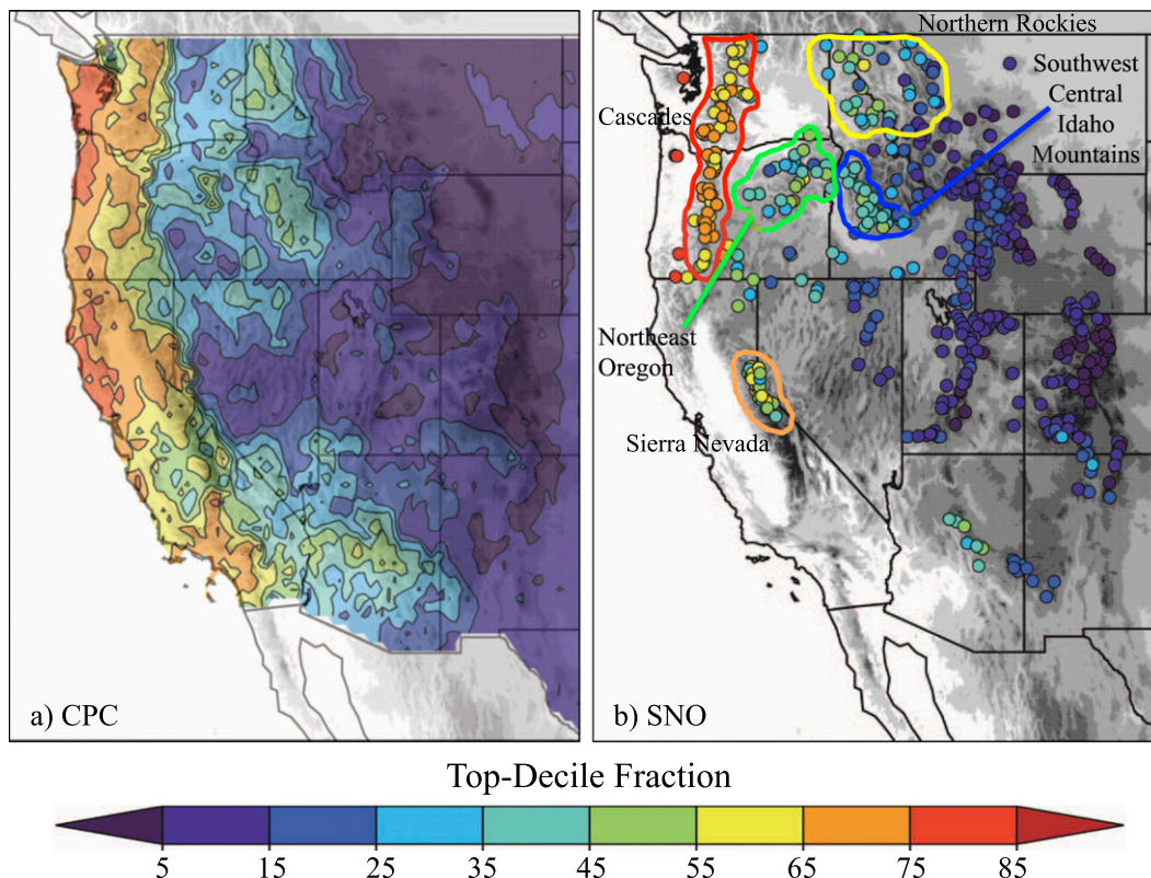
FIG. 11. As in Fig. 8, but for top-decile fraction (i.e., the fraction of top-decile 24-h precipitation events associated with ARs).
