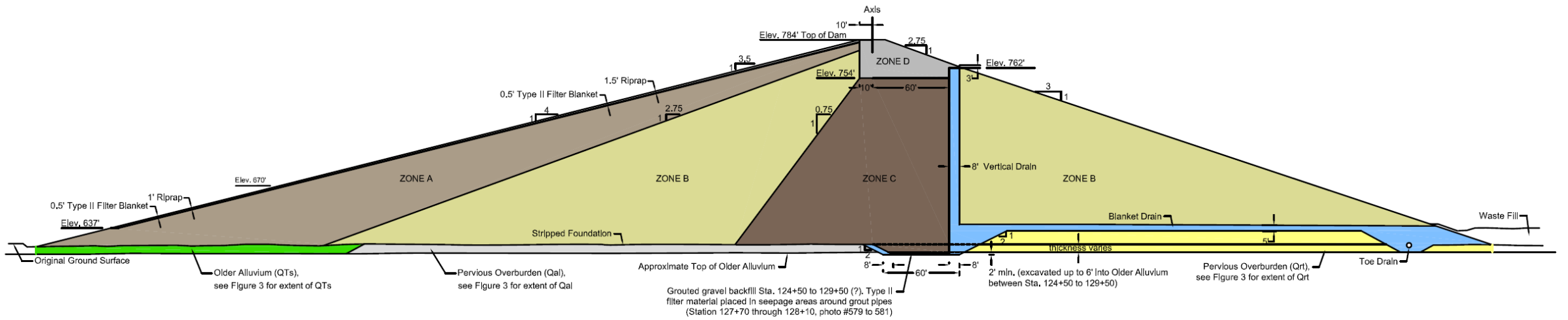
TYPICAL RIVER SECTION Station 124+10± to Station 126+00±
