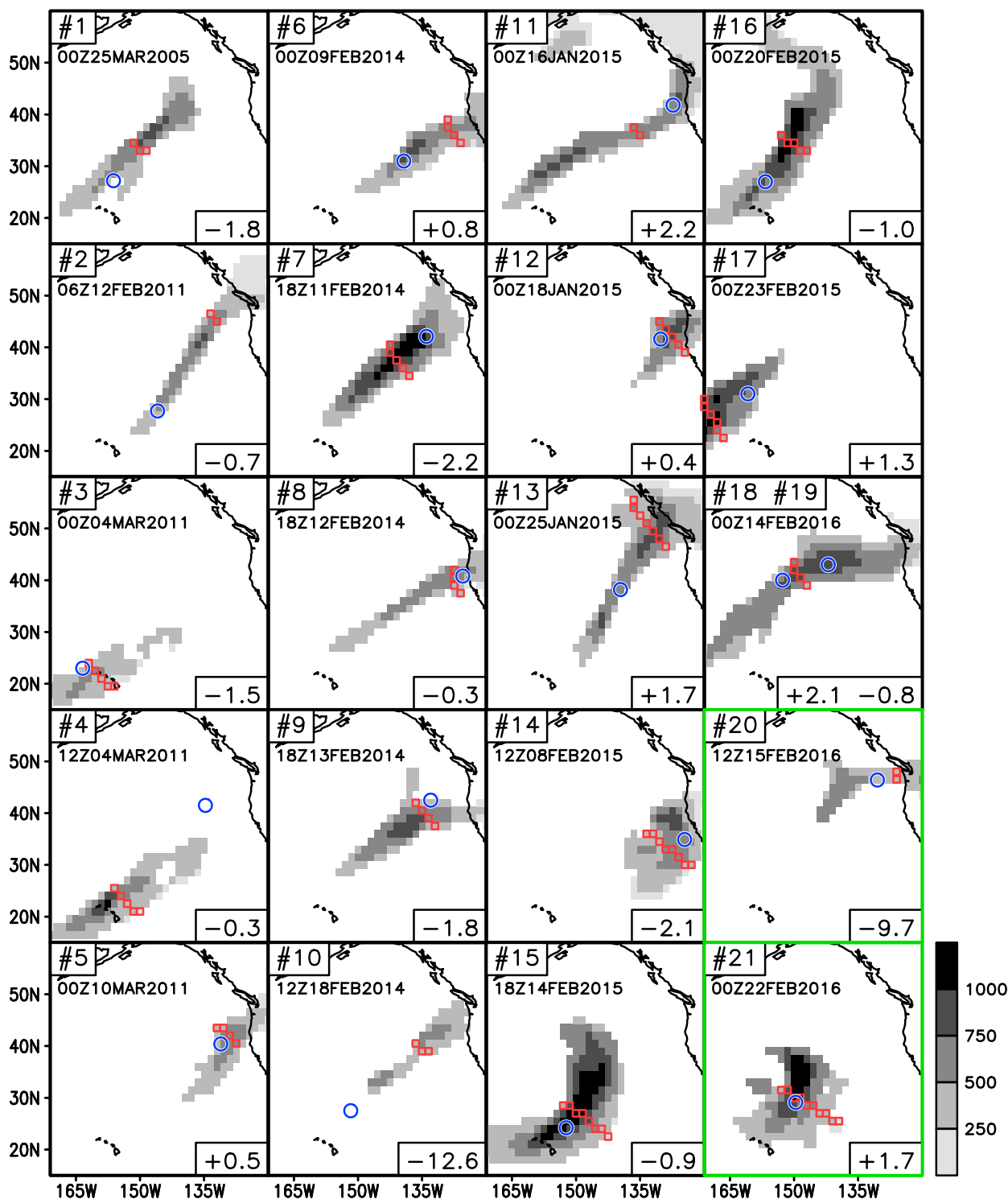
FIG. 3. The 20 ERA-Interim reanalysis ARs corresponding to the 21 dropsonde-observed AR transects. The numbering of the transect indicated in the top left of each panel is as in Ralph et al. (2017b) . Shown in each case is the 6-h step (also indicated in the top left of each panel) of the reanalysis AR (IVT magnitude in shading; \text{kg m}^{-1} \text{s}^{-1} ; transect in red) closest in time to the midpoint of the dropsonde transect (blue). Two of the 21 dropsonde transects (18 and 19) correspond to the same 6-h step of the reanalysis AR (third panel in the last column). Also indicated in each panel is the time difference (h) between the closest 6-h step of the reanalysis and the midpoint of the dropsonde transect (as a representation of the observation time), with positive/negative signs representing whether the reanalysis lags/leads the observation. Panels outlined in green show “new” ARs detected by tARget version 2 compared to the original version.
