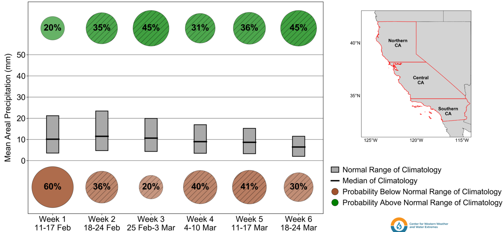
Central CA Subseasonal Precipitation Outlook Issued: 10 Feb 2025 MJO Phase 6 WQBO
