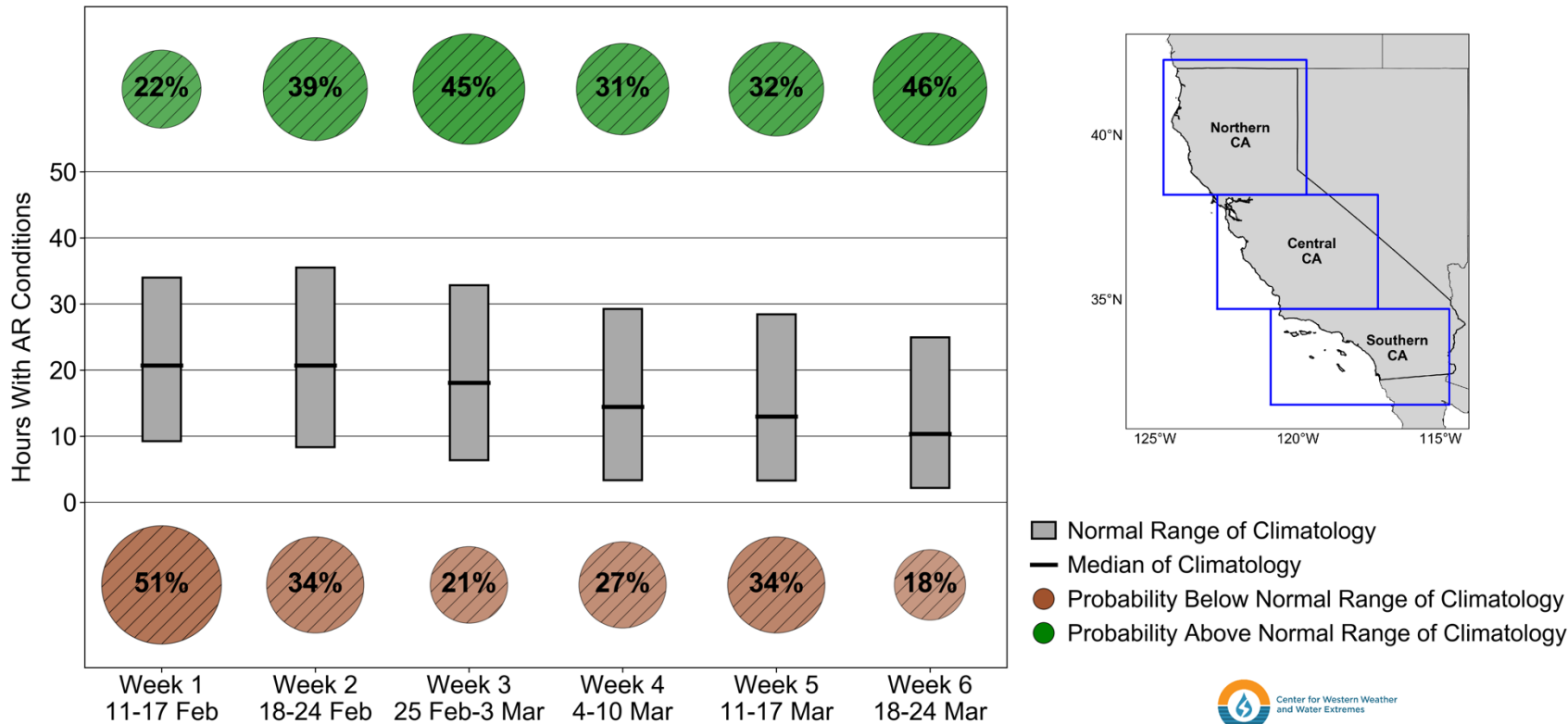
Central CA Subseasonal AR Occurrence Outlook Issued: 10 Feb 2025 MJO Phase 6 WQBO
